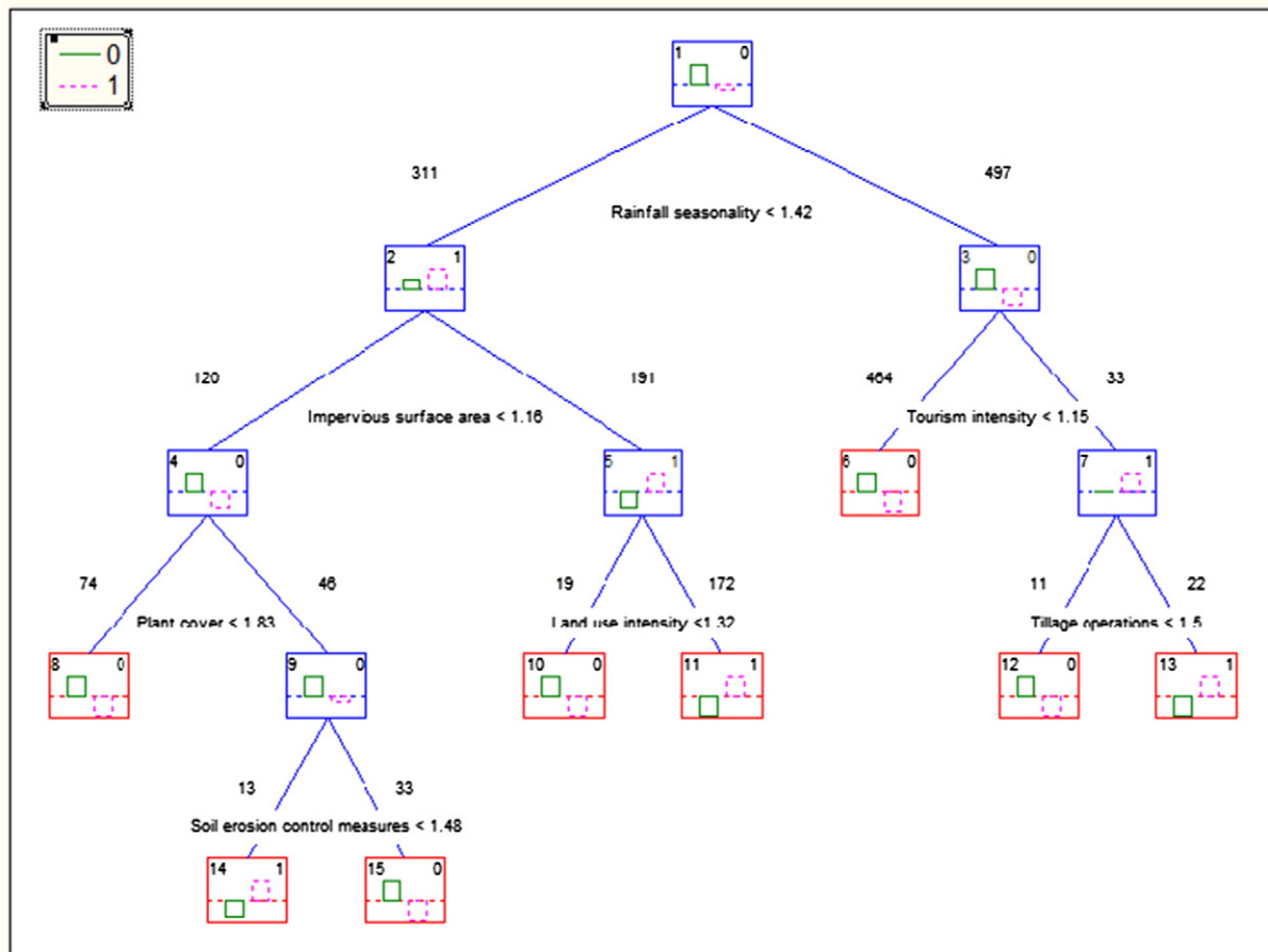
Fig. 2. Classification tree illustrating the most important drivers of land abandonment in the ten investigated study sites.
