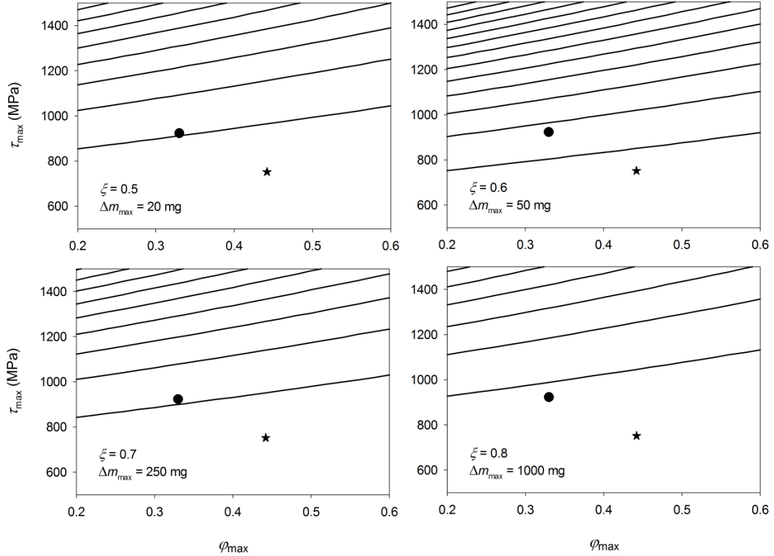
Figure 4. Contour plots of the bridging threshold. Panels represent, for different values of \xi , the relationship between the bridging threshold, m_{\max} , and the elastic properties of minor ampullate silk, \tau_{\max} and \phi_{\max} , in a wide region that probably includes the true values for most species. The properties of minor ampullate silk in A. trifasciata (star) and A. argentata (circle) are indicated for comparison. Within each panel, the bottom line represents the set of points where the bridging threshold is m_{\max} = \Delta m_{\max} . As we move upwards within each panel, lines represent the set of points where the bridging threshold is m_{\max} = 2 \cdot \Delta m_{\max} , m_{\max} = 3 \cdot \Delta m_{\max} , and so on. The values of \xi and \Delta m_{\max} are given in the lower-left corner of each panel. Bridging thresholds have been calculated from equation 6, with \beta = 2 and k = 0.3 .
